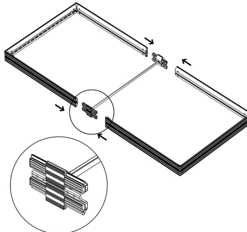
Installing key bar
