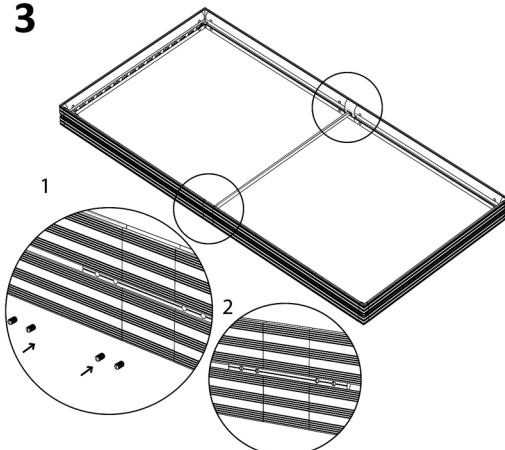
Screw fittings for thr straight connectors
